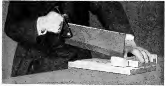
Fig. 4. Sawing Cross Grain on Bench Hook with Back or Handy Saw.
